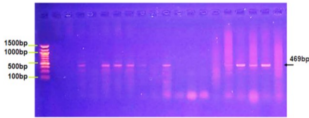
Figure 1: Molecular positive result of T. gondii infection according to BI gene (469 bp) analysis.
